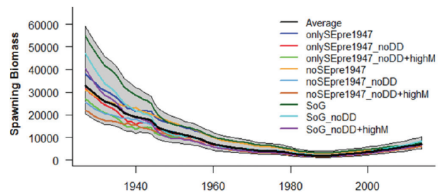
Figure 2. Posterior mean estimates of spawning biomass (in tonnes) over time for a scenario-averaging approach (solid black line). Grey shading shows the 5 th and 95 th percentiles of the scenario-averaged trajectory, while the multi-coloured solid lines show the posterior median estimates from each of the nine individual scenarios. Figure and caption from DFO 2015/014 1 .
